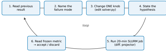
FIGURE 2 | The agentic autoresearch loop and its provenance. The agent reads the previous result, names the failure, changes one thing, states a hypothesis, runs one short cluster job grounded in the same differentiable fan-beam projector, reads the frozen calibrated-headroom metric, and accepts or discards the change. Every iteration writes an immutable record (configuration, reconstruction, metric, comparison figure).
