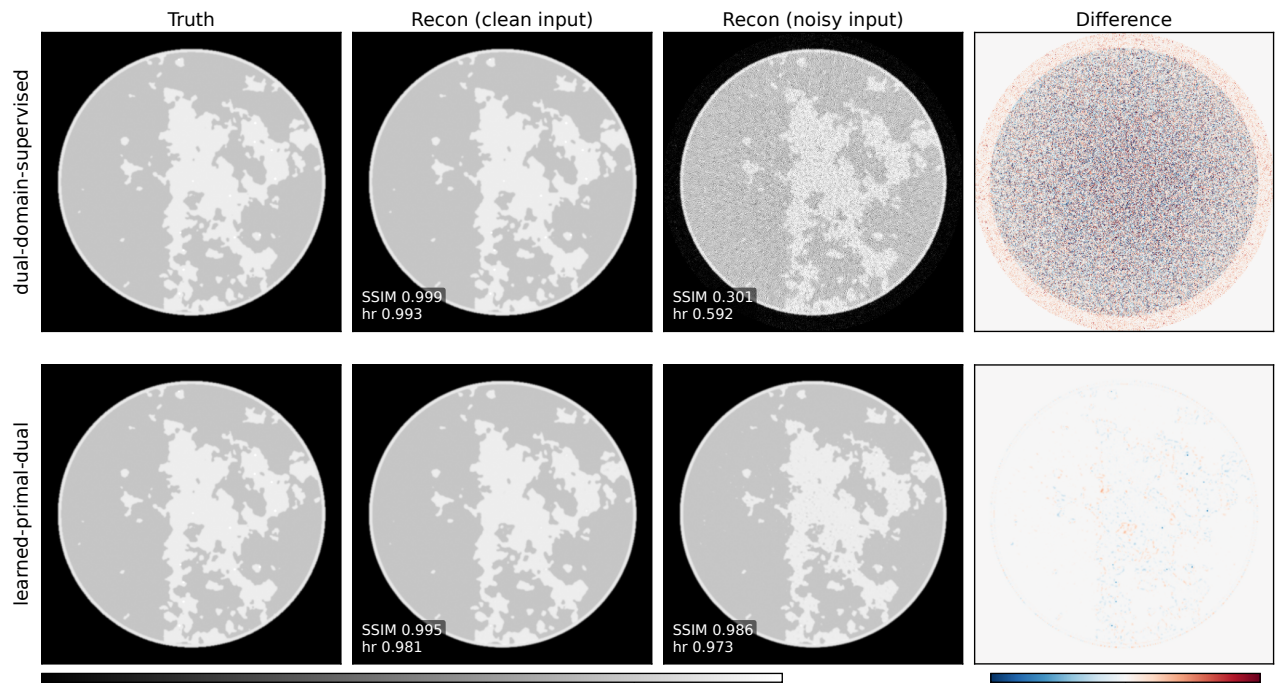
FIGURE 5 | Example reconstructions behind the reversal, for the two methods at opposite ends of it. Rows: the noiseless champion dual-domain-supervised (a supervised image-domain denoiser) versus learned-primal-dual (in-loop physics). Columns: ground truth, reconstruction from the clean input, reconstruction from the noisy input ( I_0 = 10^5 , same trained model, no retraining), and the difference to truth. Per-case SSIM and hr are annotated on each reconstruction; these are single-case values and differ from the 200-case board means in Table 4. On clean inputs both are near-perfect. Under mild input noise the supervised denoiser collapses (single-case SSIM 0.999 \rightarrow 0.301), spraying structured error across the field of view, while the physics-in-the-loop primal-dual method holds (SSIM 0.995 \rightarrow 0.986). This is the pixel-level face of the ranking reshuffle in Figure 4 and Table 4.
