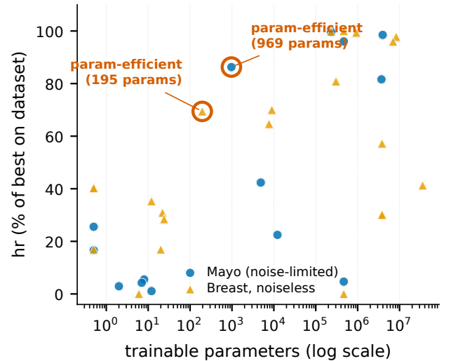
FIGURE 3 | Accuracy versus parameter count for both datasets (Mayo and breast noiseless). To overlay the two different hr scales, each solver’s hr is normalized to the percent of the best hr reached on its own board. The agent’s compact recombination solver is ringed: 969 parameters on Mayo, 195 on breast. It reaches the top accuracy tier at ~1–2 % of the parameters of the variational network.
