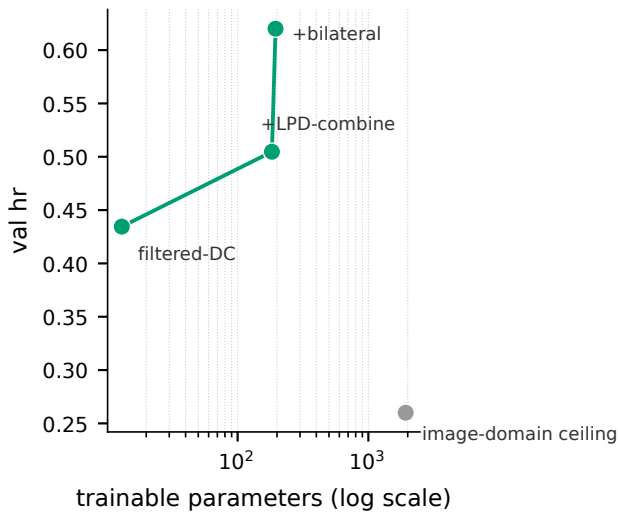
FIGURE S2 | Breast parameter/headroom Pareto front from the recombination search. The filtered data-consistency step breaks the image-domain ceiling at 13 parameters; the final design reaches the variational-network tier at 195 parameters.
