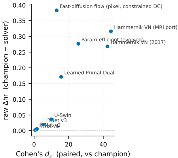
FIGURE S3 | Effect size on the breast board ( n = 200 ): Cohen's d_z versus raw \Delta hr against the champion, one point per solver. Large |d_z| at n = 200 is why the breast board separates cleanly, unlike the n = 5 Mayo board.
