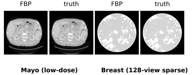
FIGURE 1 | Example slices from the two problems, each showing the FBP input the solvers start from and the ground truth. Left: Mayo low-dose CT, where quantum noise (visible graininess) is the bottleneck. Right: the 128-view sparse-view breast phantom, where undersampling produces streak artifacts. Images are windowed for display, and the FBP is intensity-calibrated to the truth as in the metric.
