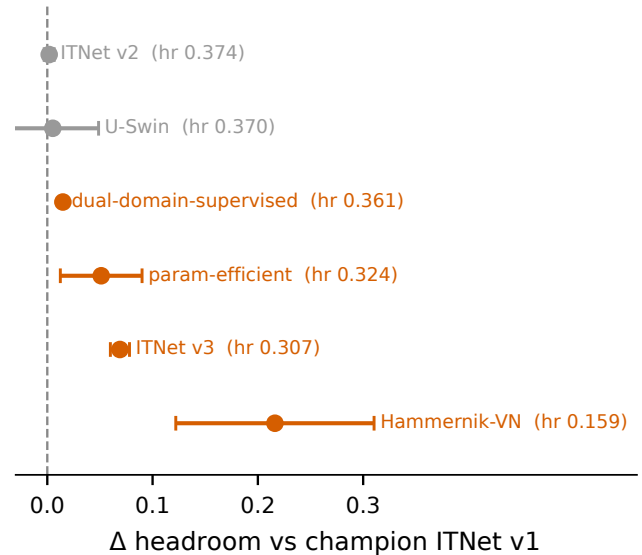
FIGURE S1 | Mayo top-solver significance: paired \Delta headroom versus the champion (ITNet v1), mean \pm 95 % CI over n = 5 patients. A confidence interval that crosses zero (grey) is a statistical tie with the champion; one that does not (red) is significantly worse. ITNet v2 and U-Swin tie; dual-domain-supervised, param-efficient, ITNet v3, and Hammernik-VN separate. Param-efficient’s interval is wide — its per-patient deficit is noisy — which is why it ties on hr at the 1 % level despite a larger mean gap than dual-domain-supervised.
