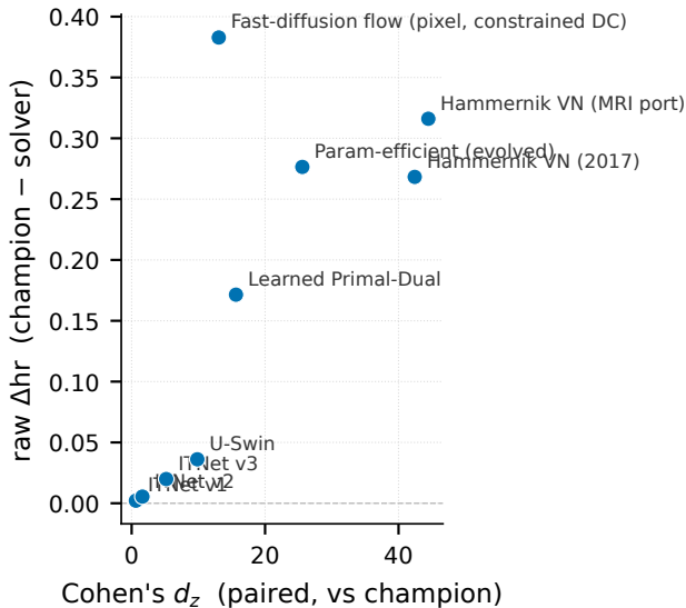
FIGURE S4 | Effect size on the breast board ( n = 200 ): Cohen's d_z versus raw \Delta hr against the champion, for the ten highest-ranked solvers (nine non-champion points; all hr > 0 ). The breast board separates cleanly because of the sample size ( n = 200 , every pairwise p < 10^{-4} ), not because the effects are large; at the n = 5 Mayo board the same-size gaps are not significant.
