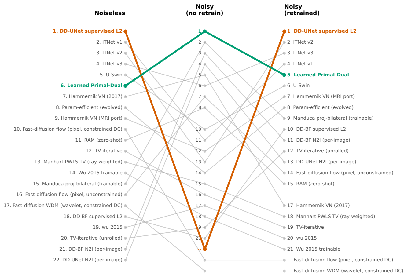
FIGURE S3 | Retraining on the noise restores the ranking. Three-column rank plot across the breast boards: noiseless (left), noisy with no retraining (middle, I_0 = 10^5 ), and noisy after retraining each solver’s clean-best configuration on matched-noise data (right); “–” marks a solver that did not clear the hr floor on that board. The noiseless champion dual-domain-supervised (orange) plunges from rank 1 to below the floor without retraining and returns to rank 1 once retrained; learned-primal-dual (green), which keeps the operator in the loop, stays near the top throughout. Grey traces show the supervised unrolled family scrambling under unseen noise and re-converging to the top after matched retraining. Spearman correlation with the noiseless ranking rises from \rho \approx 0.04 (middle) to \rho \approx 0.61 (right).
