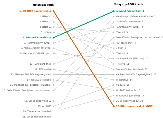
FIGURE 3 | The reversal. Paired rank plot from the noiseless breast board to the noisy breast board ( I_0 = 10^5 , same trained models, same 200 test cases, no retraining), with an arrow per method. The supervised image-domain champion collapses from rank 1 to last; the learned primal-dual method rises from mid-pack to champion; hand-crafted smoothing and in-loop physics priors rise. A small, realistic noise perturbation reorders almost the whole leaderboard.
