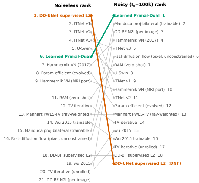
FIGURE 3 | The reversal (main result). Paired rank plot from the noiseless breast board to the noisy breast board ( I_0 = 10^5 , same trained models, same 200 test cases, no retraining), with an arrow per method. The supervised image-domain champion collapses from rank 1 to last; the learned primal-dual method rises from mid-pack to champion; hand-crafted smoothing and in-loop physics priors rise. A small, realistic noise perturbation reorders almost the whole leaderboard.
