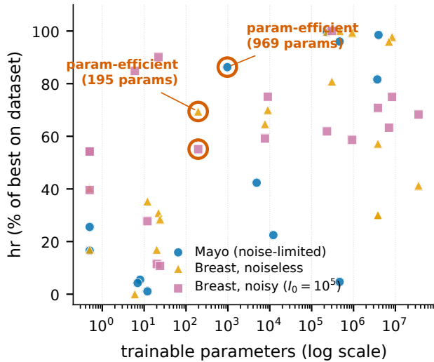
FIGURE 2 | Accuracy versus parameter count for all three boards (Mayo, breast noiseless, breast noisy). To overlay the three different hr scales, each solver's hr is normalized to the percent of the best hr reached on its own board. The agent's compact recombination solver is ringed: 969 parameters on Mayo, 195 on both breast boards. It reaches the top accuracy tier at ~1–2 % of the parameters of the variational network.
