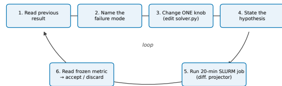
FIGURE 1 | The agentic autoresearch loop and its provenance. The agent reads the previous result, names the failure, changes one thing, states a hypothesis, runs one short cluster job grounded in the same differentiable fan-beam projector, reads the frozen calibrated-headroom metric, and accepts or discards the change. Every iteration writes an immutable record (configuration, reconstruction, metric, comparison figure).
