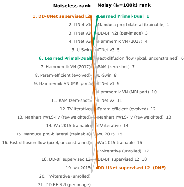
FIGURE 3 | The reversal. Paired rank plot from the noiseless breast board to the noisy breast board ( I_0 = 10^5 , same trained models, same 200 test cases, no retraining), with an arrow per method. The supervised image-domain champion collapses from rank 1 to last; the learned primal-dual method rises from mid-pack to champion; hand-crafted smoothing and in-loop physics priors rise. A small, realistic noise perturbation reorders almost the whole leaderboard.
