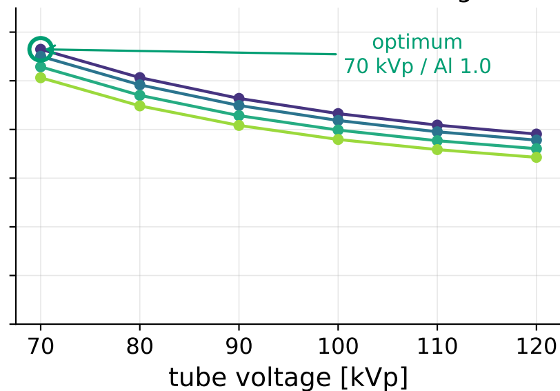
PCD - iron CNR vs tube voltage
