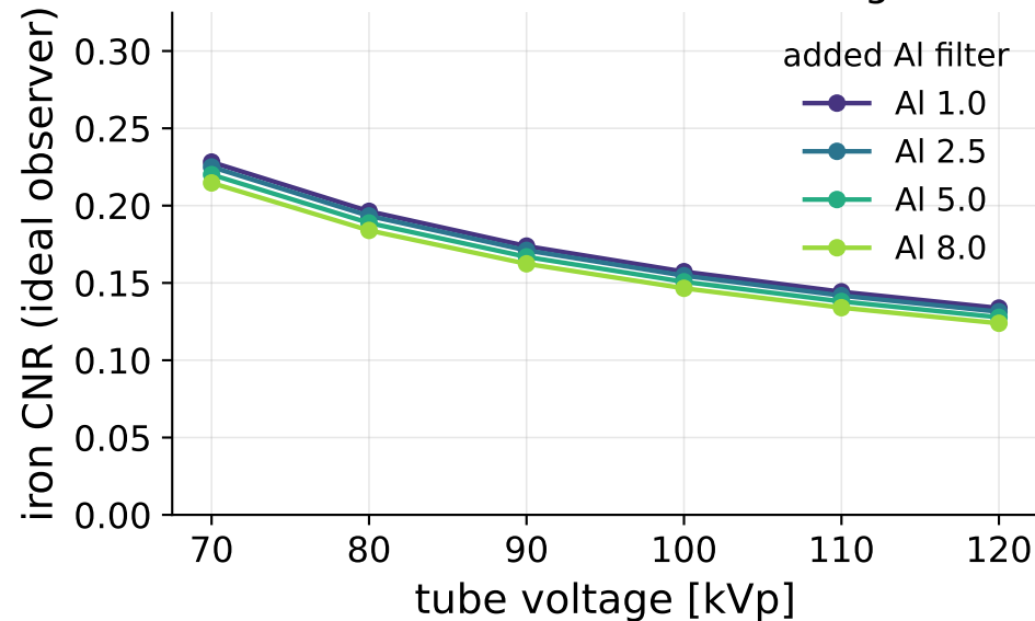
EID - iron CNR vs tube voltage
