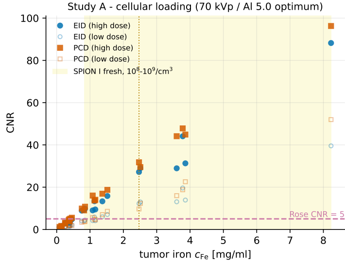
Figure 4. Study A detectability. Iron \Delta\text{HU} (left) and CNR (right) versus in-tumor iron concentration for EID and PCD, with the Rose 3 and 5 lines. The shaded band spans the three tumor cell densities ( 10^8 – 10^9 cells/cm 3 ); it shows that visibility is dominated by cell density.
