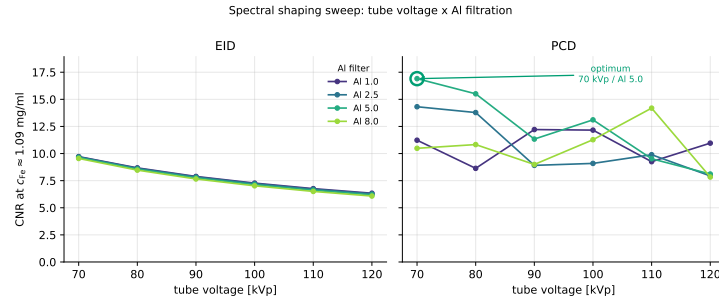
Figure 3. E2 spectral optimization. CNR versus tube voltage across aluminium filters, for EID and PCD. Lower tube voltage helps; hardening filters hurt. The selected CNR-optimal spectrum (70 kVp, Al 5 mm, PCD bin edges 10/37.5/47.5/70 keV) feeds E3–E5.
