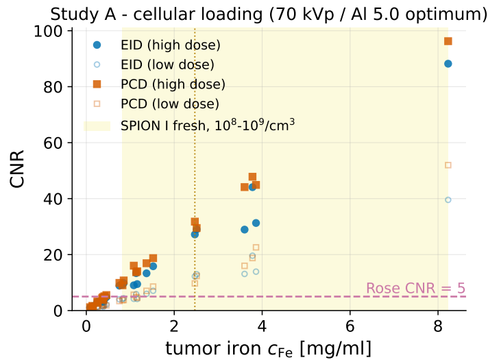
Figure 4. Study A detectability. Iron \Delta HU (left) and CNR (right) versus in-tumor iron concentration for EID and PCD, with the Rose 3 and 5 lines. The shaded band spans the three tumor cell densities ( 10^8 – 10^9 cells/cm 3 ); it shows that visibility is dominated by cell density.
