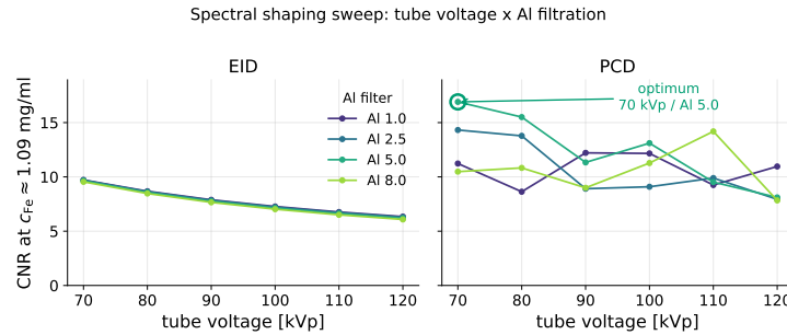
Figure 3. E2 spectral optimization. CNR versus tube voltage across aluminum filters, for EID and PCD. Lower tube voltage helps; hardening filters hurt. The selected CNR-optimal spectrum (70 kVp, Al 5 mm, PCD bin edges 10/37.5/47.5/70 keV) feeds E3–E5.
