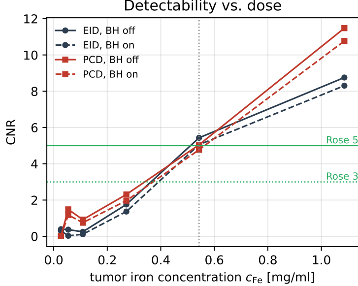
Figure 6. CNR versus dose for both detectors, beam-hardening on/off, with the Rose 3 and 5 lines. The realistic dose (dotted) lands on the Rose-5 boundary.
