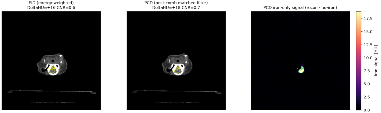
Figure 8. E5 three-dimensional verification in real anatomy. A cervical slice of the post-mortem RabbitCT rabbit, reconstructed with cone-beam FDK at the E2 optimum (70 kVp, Al 5 mm), with an inserted SPION I fresh tumor ( c_{Fe} = 2.47 mg Fe/ml). Left: energy-integrating detector (+16 HU). Middle: photon-counting detector, post-combination matched filter (+18 HU). Right: the PCD iron-only signal (reconstruction minus a no-iron reference), which localizes the tumor while the anatomy cancels. The PCD gives the larger contrast at every iron level.
