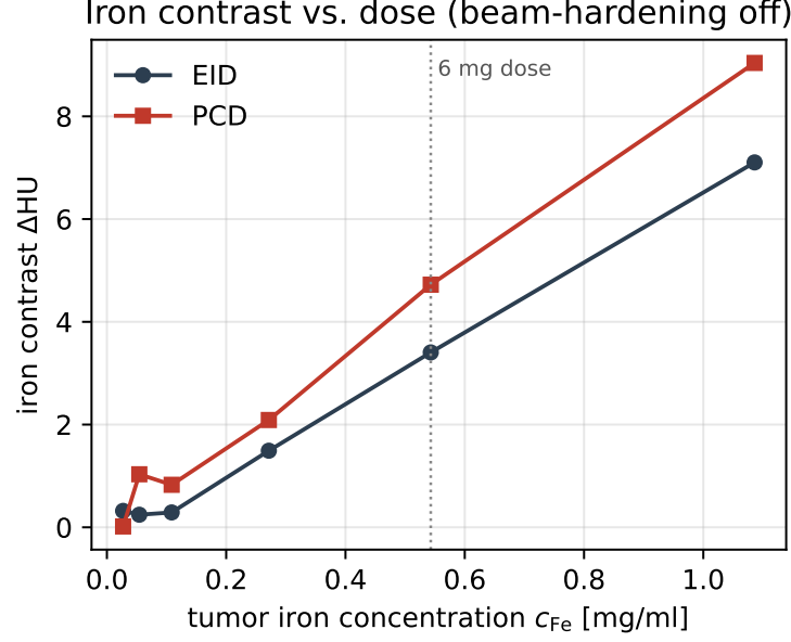
Figure 5. Iron contrast \Delta HU versus in-tumor iron concentration for the two detectors (beam-hardening off). The dotted line marks the realistic 6 mg dose.
