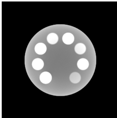
PCD - noise-free
