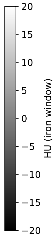
PCD - 1 realization
