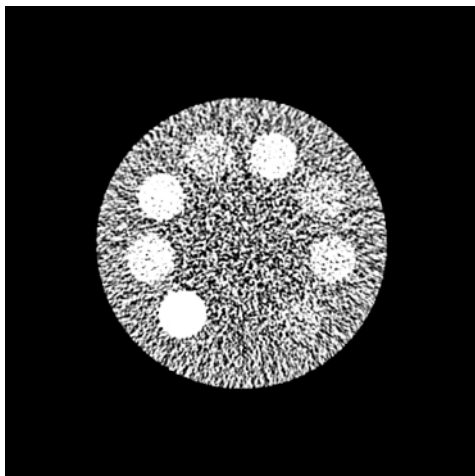
EID - 1 realization
