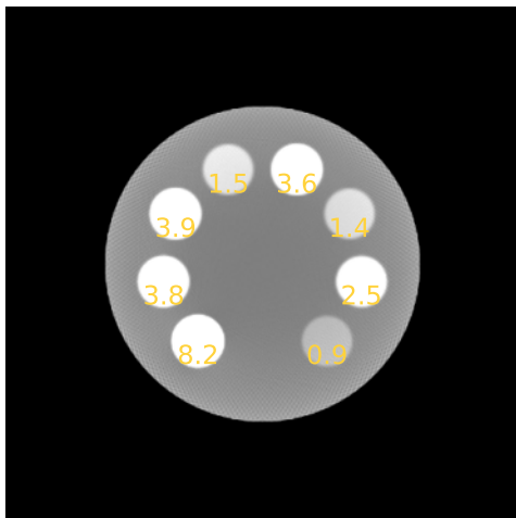
EID - noise-free
