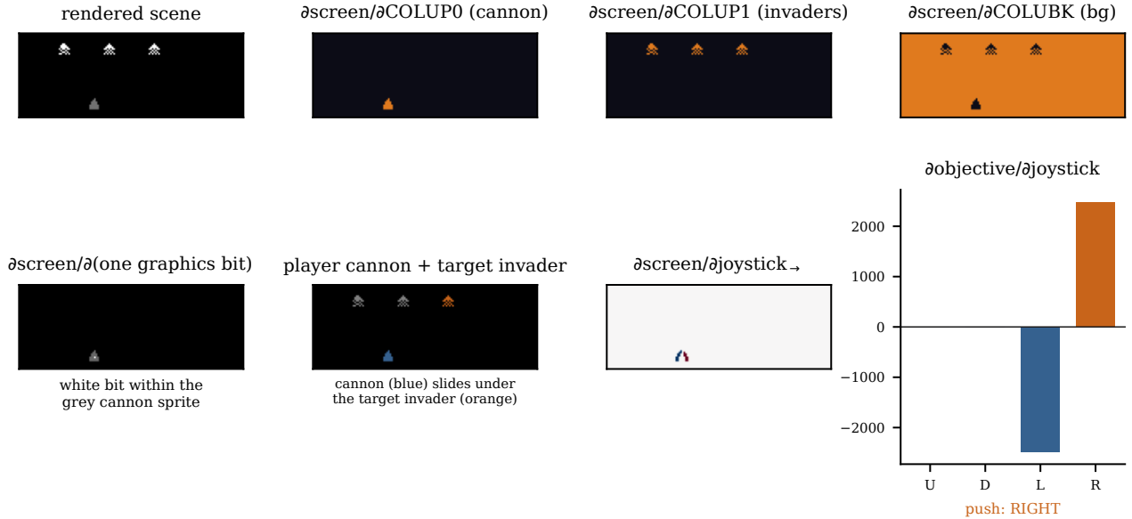
Figure 3: Qualitative XAI on a Space Invaders scene in the differentiable VCS, all computed by reverse-mode AD through JUTARI. The scene is a row of invaders (player 1, multi-copied by the NUSIZ register) and a player cannon (player 0) that moves left/right. Top: from the unmodified soft renderer, a Grad-CAM analogue— \partial\text{screen}/\partial\text{register} localises each object to exactly the pixels its register controls (the cannon via COLUP0, the invaders via COLUP1, the background via COLUBK), a localisation that can be checked against ground truth. Bottom, left to right: a single cannon graphics bit (bright, within the faint cannon outline) attributes to its own pixels once represented as a value behind a stored switch; the scene with the cannon (bottom) and the target invader it should slide under (orange); the signed \partial\text{screen}/\partial\text{joystick} saliency (a soft sampler makes the position differentiable), highlighting the cannon edges that move; and the gradient of the on-screen cannon position with respect to the four joystick directions, which correctly infers that pushing RIGHT (and not up/down) moves the cannon toward the target.
