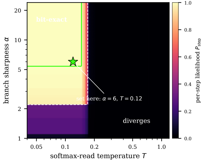
Figure 2: Overview of the per-step bit-exactness likelihood P_{\text{step}} = p_{\text{read}}(T)^p p_{\text{branch}}(\alpha)^{f_b} of the fully relaxed forward across the (\alpha, T) plane (Space Invaders). A bit-exact corner—bright, with the green contour marking P_{\text{step}}=1 —sits at large branch sharpness \alpha and small read temperature T , bounded by a gradual branch boundary (in \alpha ) and a sharp temperature boundary (in T ); the white dashed line is P_{\text{step}}=0.5 . Because P_{\text{step}} factorises, the plane is the outer combination of the two 1D profiles, and the two boundary sweeps of Table 1 are slices along the green contour’s two edges. The star marks the recommended operating point ( \alpha=6 , T=0.12 )—the corner where they cross.
