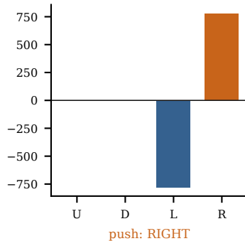
\partial \text{objective} / \partial \text{joystick}
