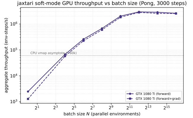
Figure 5: JAXTARI soft-mode GPU throughput vs. batch size N (Pong, 3,000 steps; commodity GTX 1080 Ti). Forward and forward+gradient both rise \sim 1200\times from N=1 to a peak near N=4096 ( \sim 3\text{M} env-steps/s, \sim 50\times the CPU vmap asymptote, dotted), then roll off as the device saturates—the 256-way lax.switch all-branch dispatch parallelises across lanes on the GPU where it serialises on the CPU.
