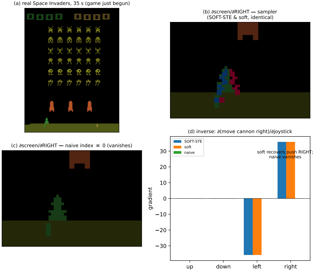
Figure 5: Ground-truth gradients on the real Space Invaders ROM in the differentiable VCS. (a) the live game 35 s after boot—the scene the real ROM renders, pixel-exact to XITARI . (b) the screen’s directional derivative with respect to the RIGHT joystick, recovered by a differentiable sampler over the player-cannon position (a sub-pixel bilinear kernel, as in spatial-transformer networks); it lights exactly the cannon edges that move. Because soft mode is forward-exact (Theorem 1), this gradient is identical for SOFT-STE and the soft (relaxed) variant (the leaky, past-boundary variant is studied in the supplement). (c) the naive gradient runs through the discrete sprite-position index and is identically zero—it would wrongly report “the joystick does not affect the screen.” (d) the inverse problem, \partial(\text{move cannon right}) / \partial \text{joystick} : SOFT-STE and soft recover the control mapping (push RIGHT , not up/down), while the naive gradient vanishes. Every recovered quantity can be checked against the known wiring—the whole point of a ground-truth substrate.
