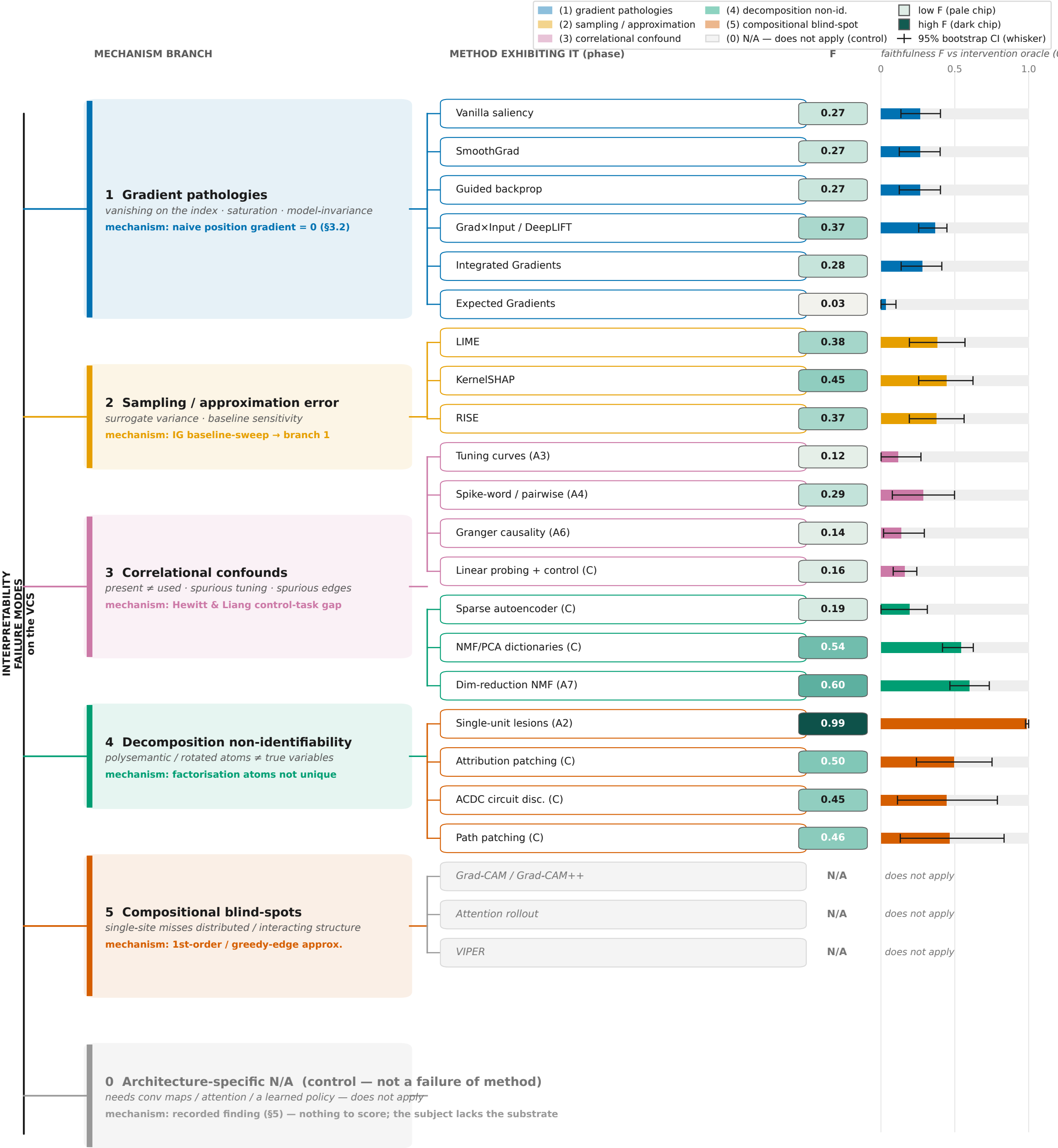
A taxonomy of interpretability failure modes on the VCS, by underlying mechanism (full version — Supplement)
