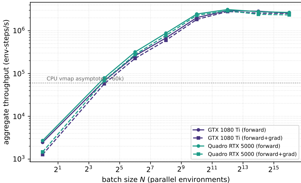
jaxtari soft-mode GPU throughput vs batch size (Pong, 3000 steps)
