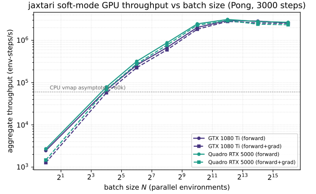
Figure 5: JAXTARI soft-mode GPU throughput vs. batch size N (Pong, 3,000 steps; two commodity GPUs, GTX 1080 Ti and Quadro RTX 5000). Forward and forward+gradient both rise \sim 1200\times from N=1 to a peak near N=4096 ( \sim 3\text{M} env-steps/s, \sim 50\times the CPU vmap asymptote, dotted), then roll off as the device saturates—the 256-way lax.switch all-branch dispatch parallelises across lanes on the GPU where it serialises on the CPU.
