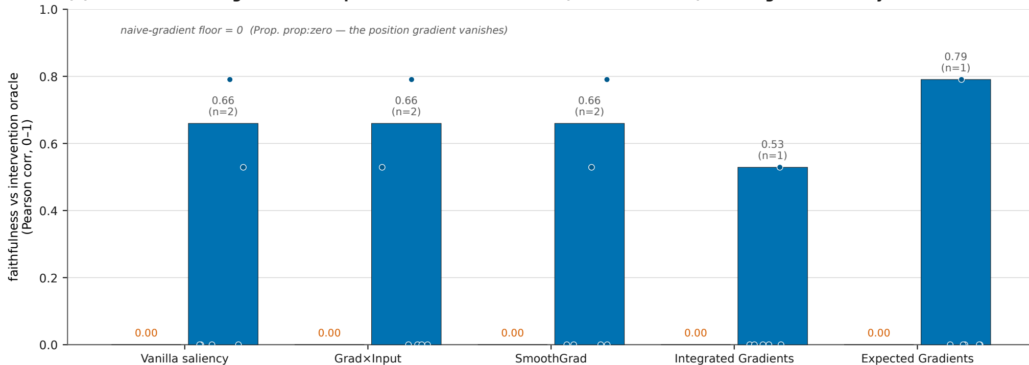
(a) Position/index regime: the sampler RESTORES faithfulness (0 → off the floor) for the gradient family
