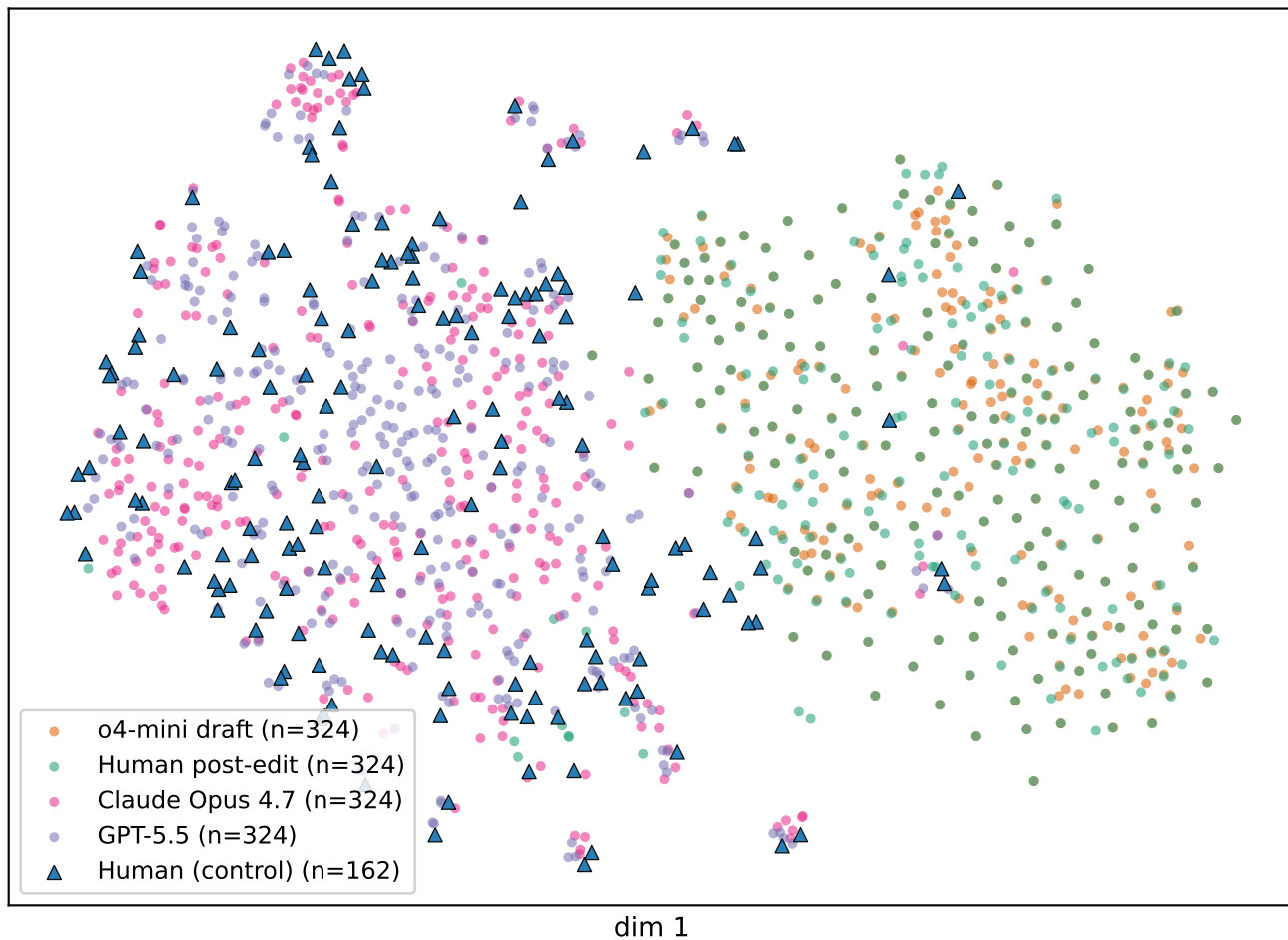
Figure 12b: t-SNE(2) of LUAR embeddings, colored by approach
