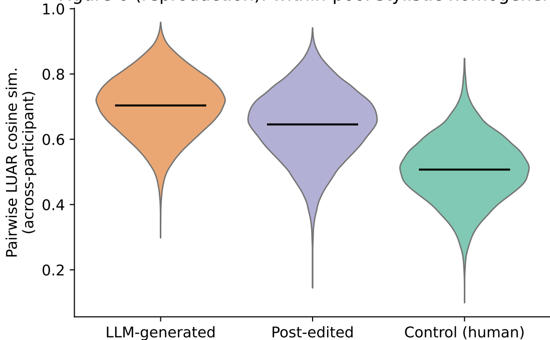
Figure 6 (reproduction): within-pool stylistic homogeneity
