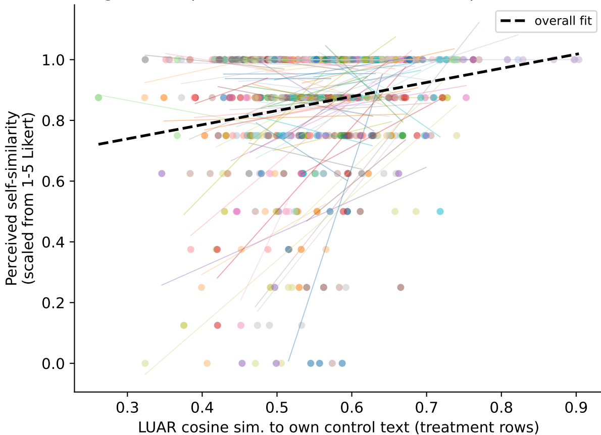
Figure 8 (reproduction): rmcrr r=+0.244 , p=3.633e-09
