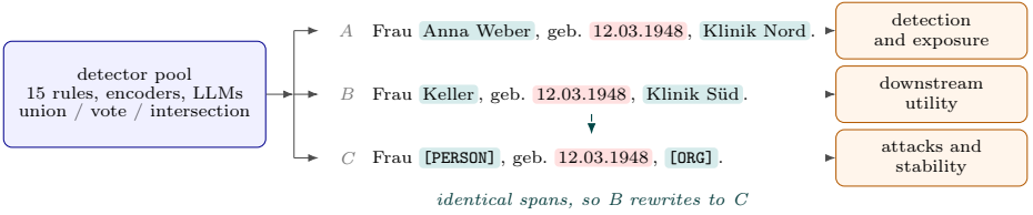
Fig. 1: One detector span set, three release conditions, on an invented header line. Identifiers (teal) become surrogates in B and typed placeholders in C; dates (red) pass through. A surrogate replaces a whole span, so a two-token name becomes one. B and C replace identical spans.
