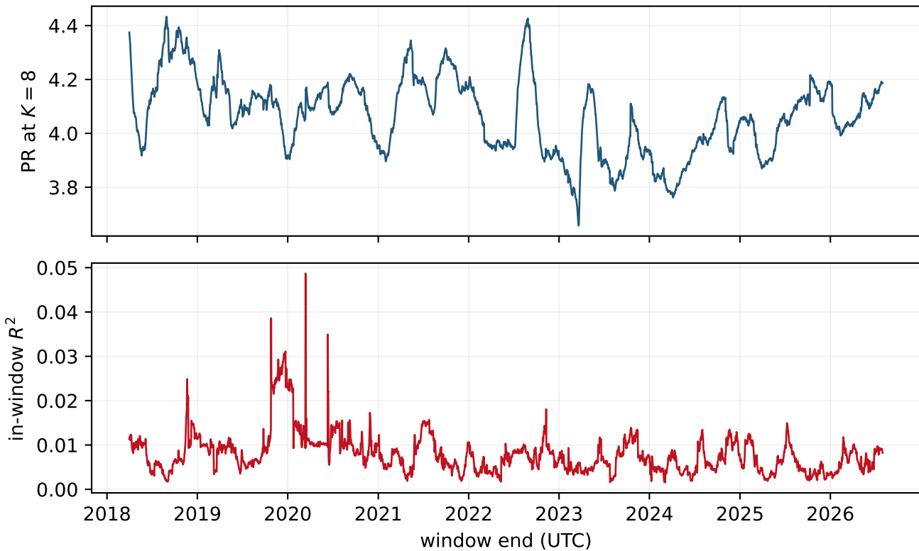
90-day rolling participation ratio and OLS fit (descriptive only)
