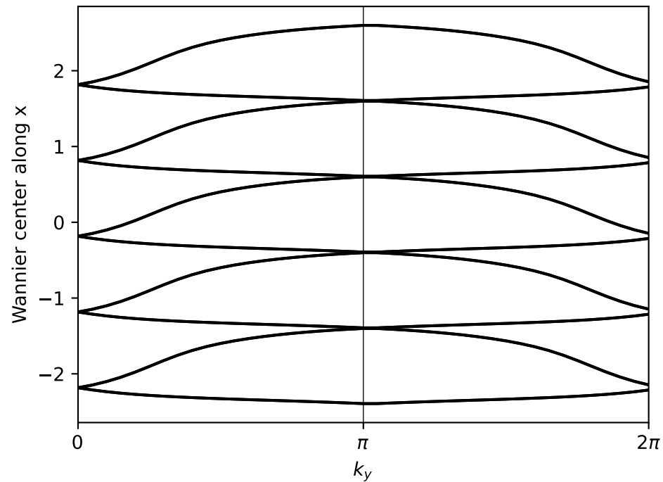
1D Wannier centers: Intralayer Case
