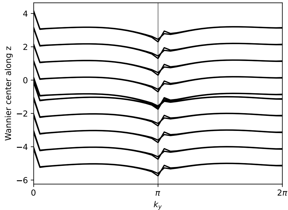
1D Wannier centers: Interlayer Case
