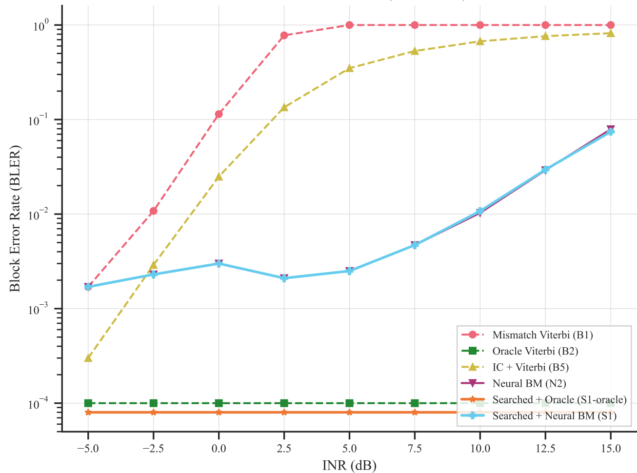
Robustness to interference (SNR = 5 dB)
