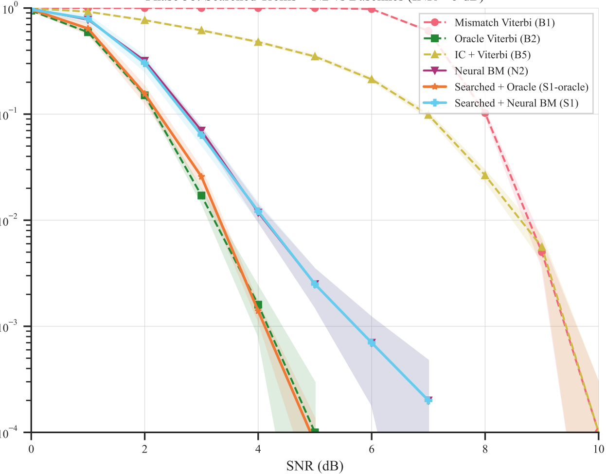
Phase 3b: Searched Trellis + N2 vs Baselines (INR = 5 dB)
