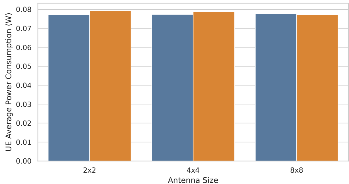
Urban Macro: UE Average Power Consumption (W) by Antenna and Channel Mode
