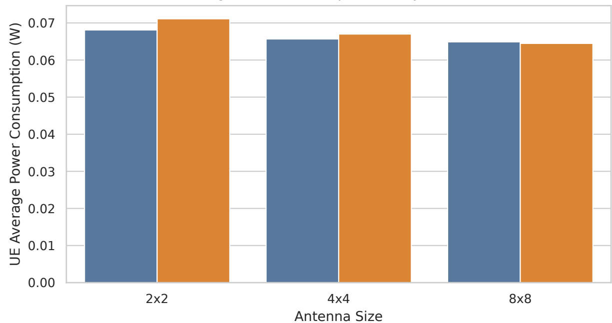
Urban Micro: UE Average Power Consumption (W) by Antenna and Channel Mode
