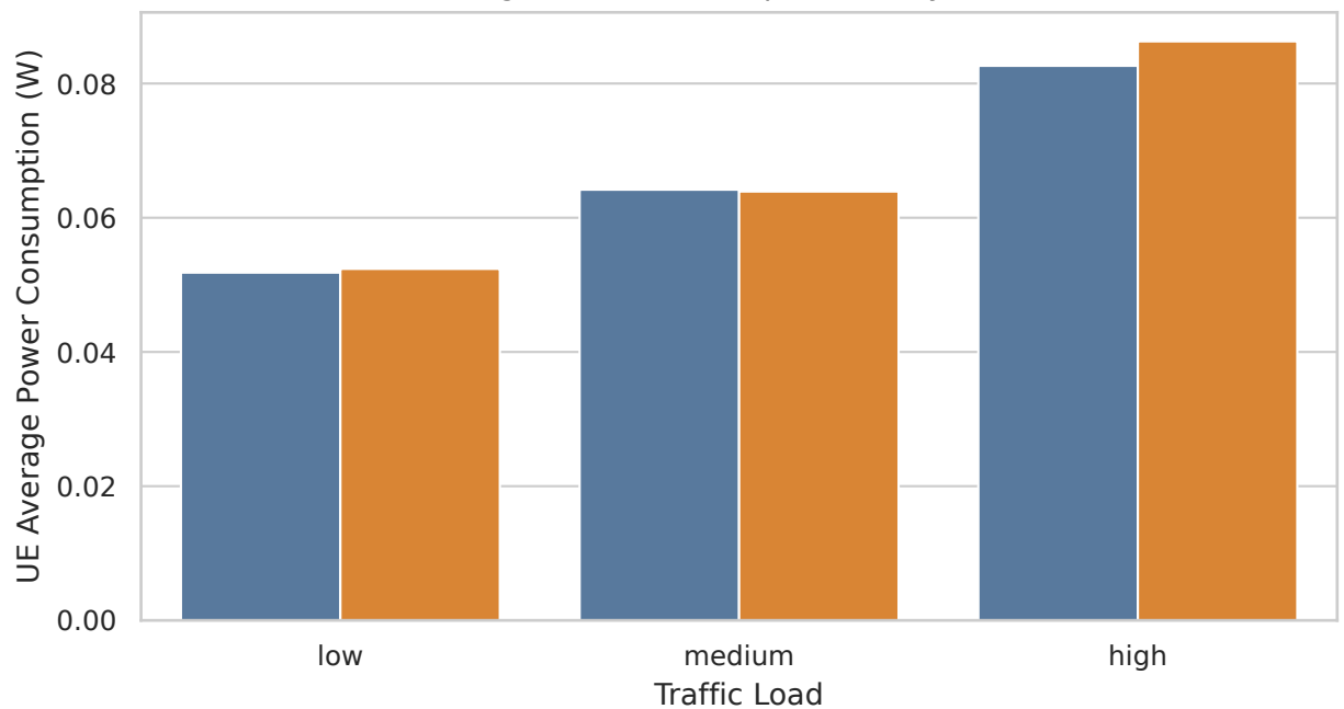
Urban Micro: UE Average Power Consumption (W) by Load and Channel Mode
