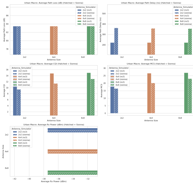
Fig. 10. Urban macro propagation-related metrics by channel mode and gNB array size.
