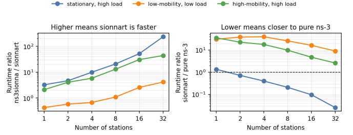
Fig. 3. The left graph shows the ratio of ns3sionna runtime to sionnart runtime. The right graph is the ratio of sionnart runtime to pure_ns-3 baseline runtime.
