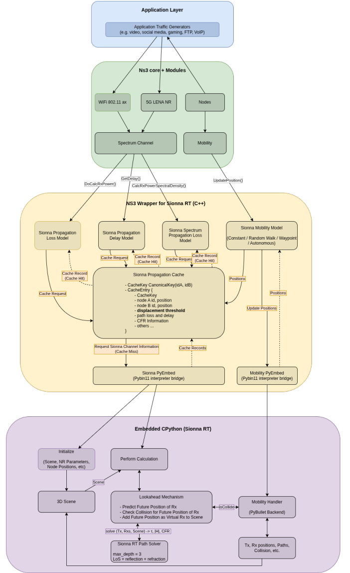
Fig. 1. Architecture of the integrated simulation framework.
