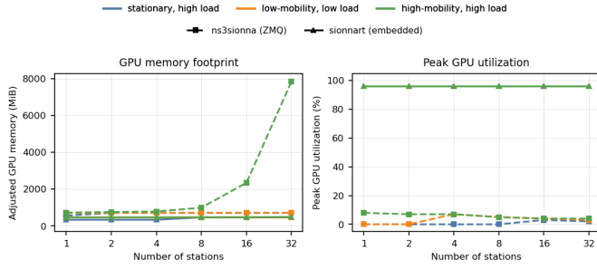
Fig. 4. Reported GPU memory footprint and peak utilization for the two Sionna-backed backends.
