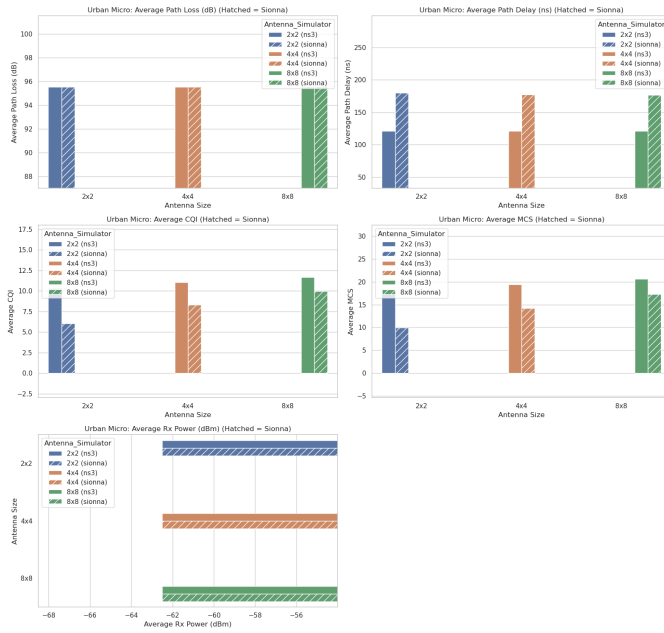
Fig. 13. Urban micro propagation-related metrics by channel mode and gNB array size.
