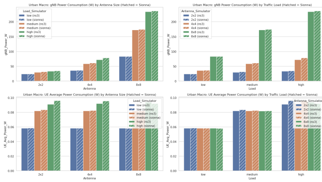
Fig. 11. Urban macro energy consumptions of gNB and UEs by array size, and traffic load.
