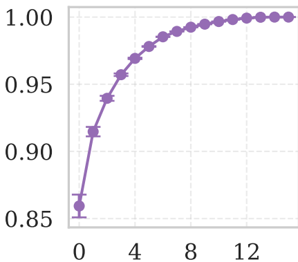
FMNIST
