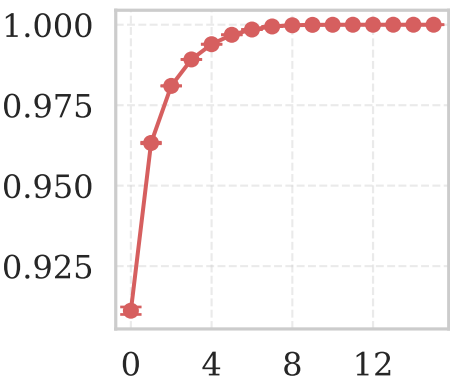
CIFAR-10
