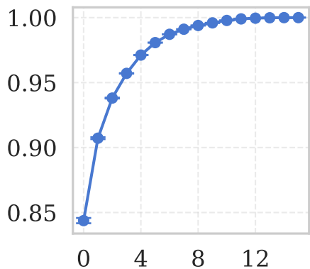
GIST
