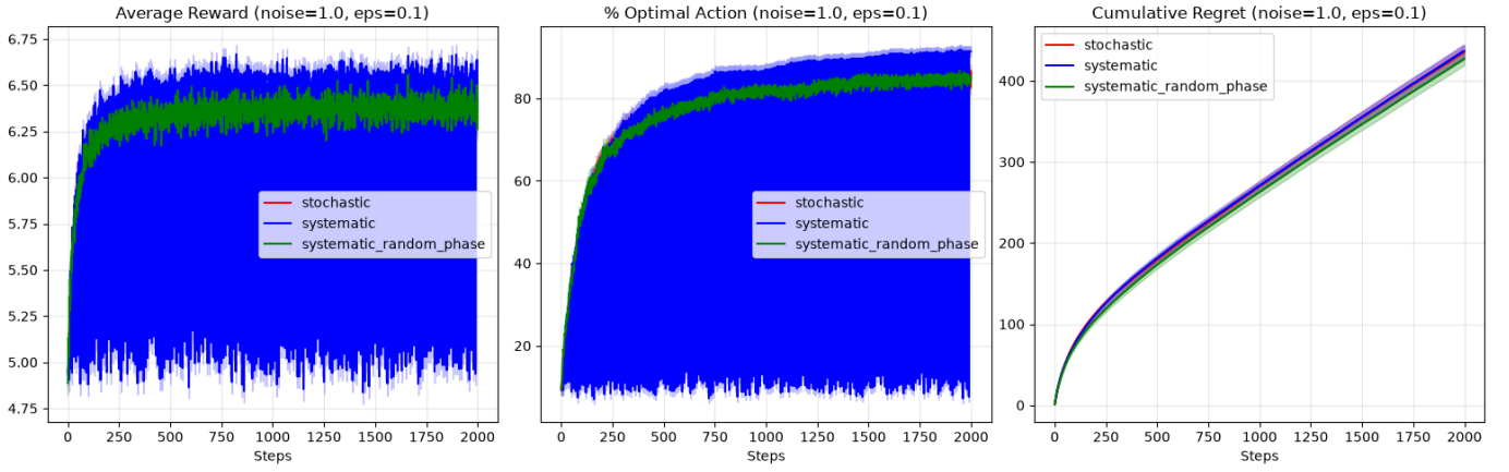
Fig. 3. \sigma = 1 , \epsilon = 0.1
