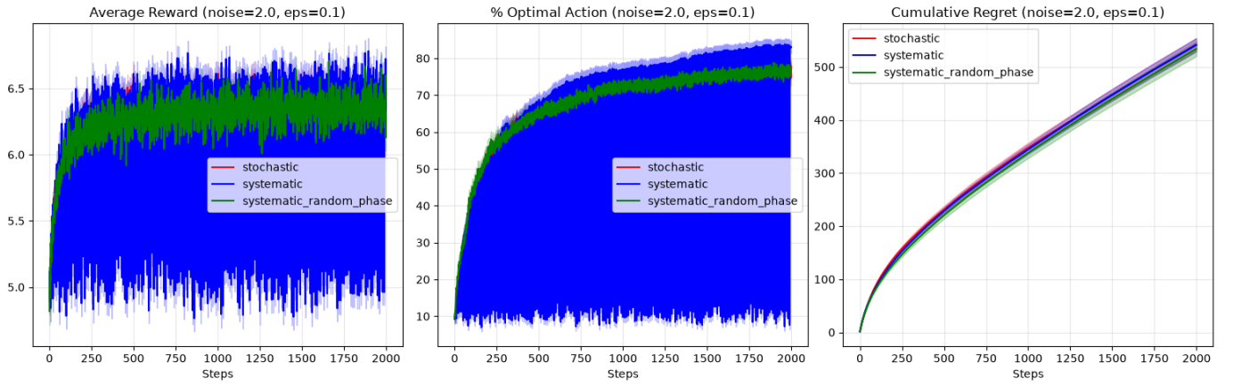
Fig. 5. \sigma = 2, \varepsilon = 0.1
