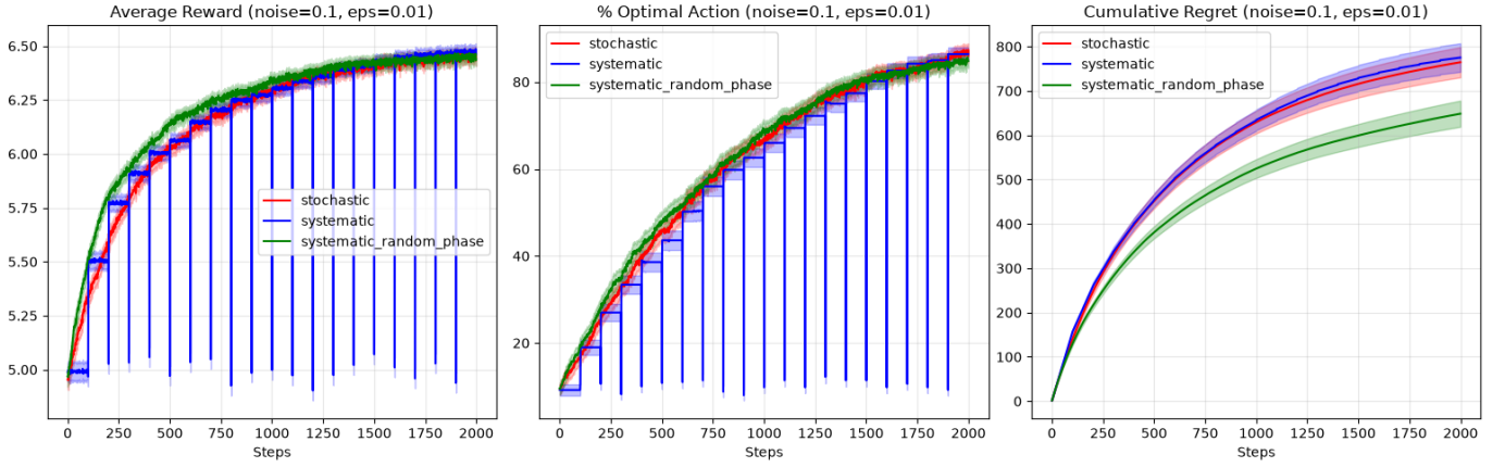
Fig. 2. \sigma = 0.1, \epsilon = 0.01
