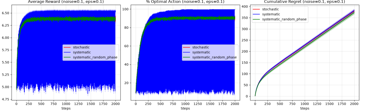
Fig. 1. \sigma = 0.1, \epsilon = 0.1
