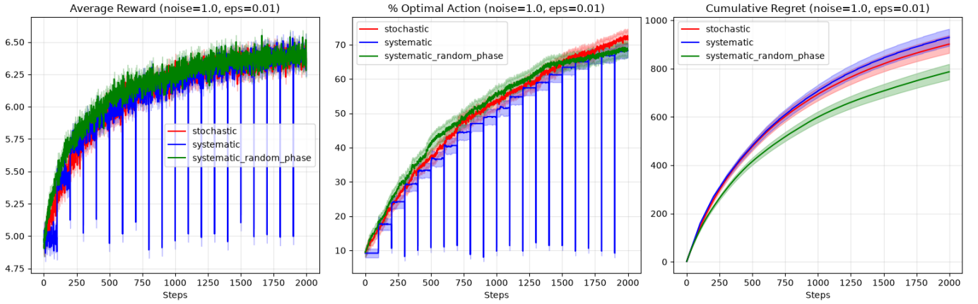
Fig. 4. \sigma = 1 , \epsilon = 0.01
