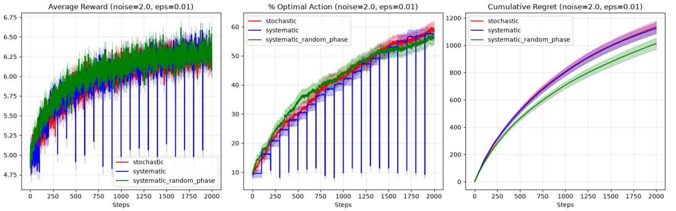
Fig. 6. \sigma = 2, \varepsilon = 0.01
