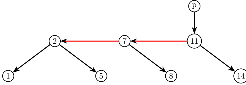
Figure 7: Inserting a new node — left child, uncle is BLACK
