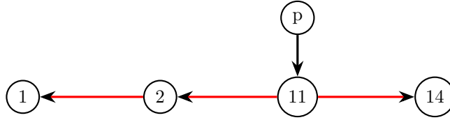
Figure 3: Inserting a new node — uncle is RED
