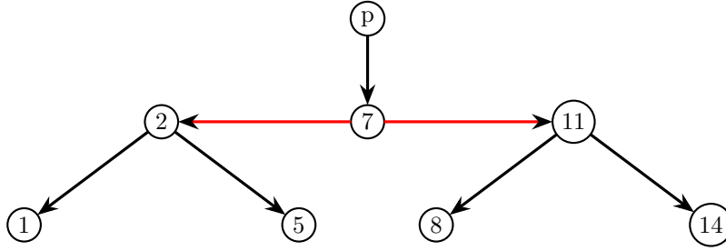
Figure 6: Fix of Case 2.1 violation
