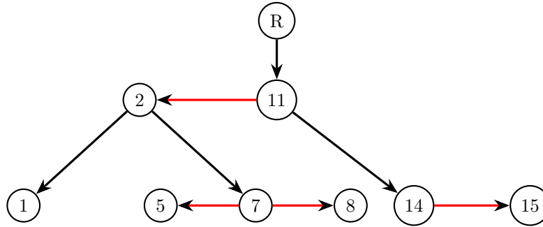
Figure 1: A Red-Black tree
