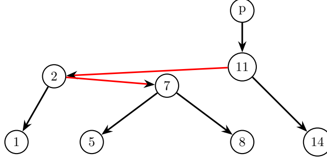
Figure 5: Inserting a new node — zig-zag, uncle is BLACK
