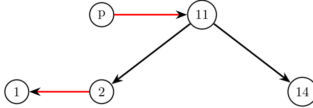
Figure 4: Fix of Case 1 violation
