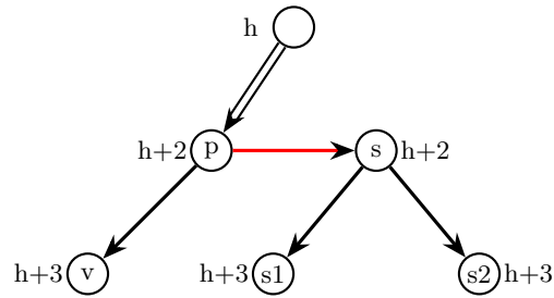
Figure 16: Fix of Case D.4
