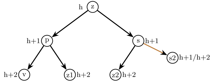
Figure 12: Fix of Case D.2
