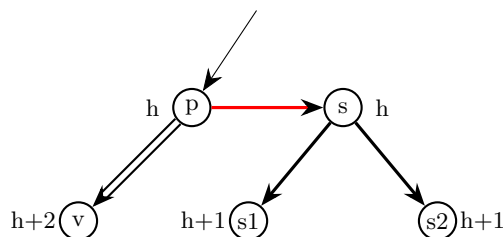
Figure 17: Case D.5: BLACK sibling with BLACK children and BLACK parent
