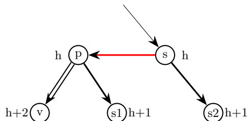
Figure 18: Handling of Case D.5
