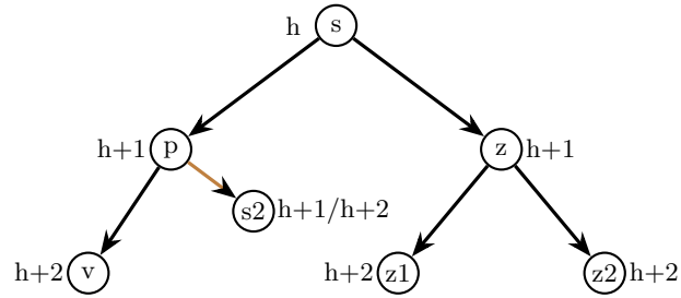
Figure 10: Fix of Case D.1
