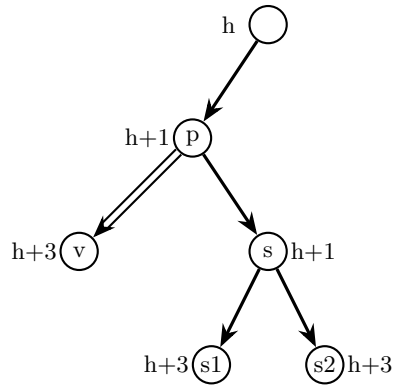
Figure 15: Case D.4 : BLACK sibling with BLACK children and BLACK parent
