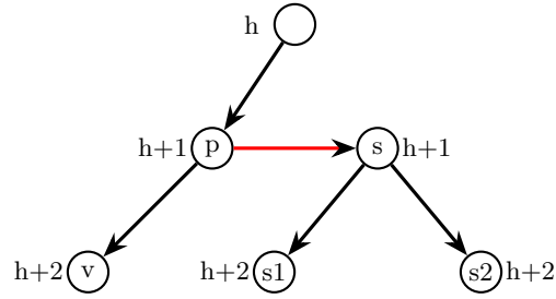
Figure 14: Fix of Case D.3
