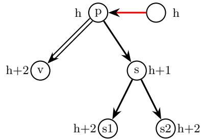
Figure 13: Case D.3: BLACK sibling with BLACK children and RED parent
