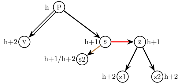
Figure 9: Case D.1 : BLACK sibling with a right RED child
