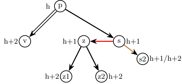
Figure 11: Case D.2: BLACK sibling with a left RED child
