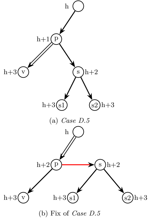
Figure 13: Case D.5: BLACK sibling with BLACK children and parent
