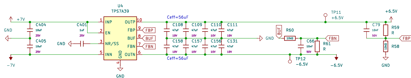
+/-7V to +/-6.5V LDO
