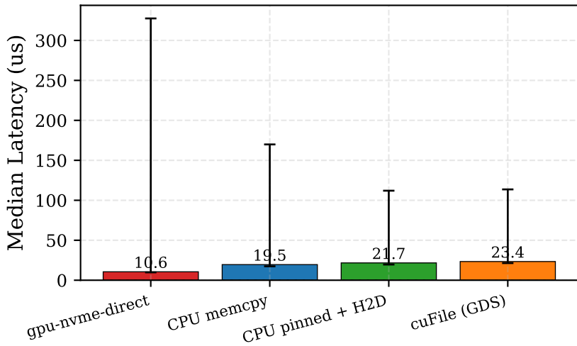
Per-Operation Latency at 4KB, QD=1
