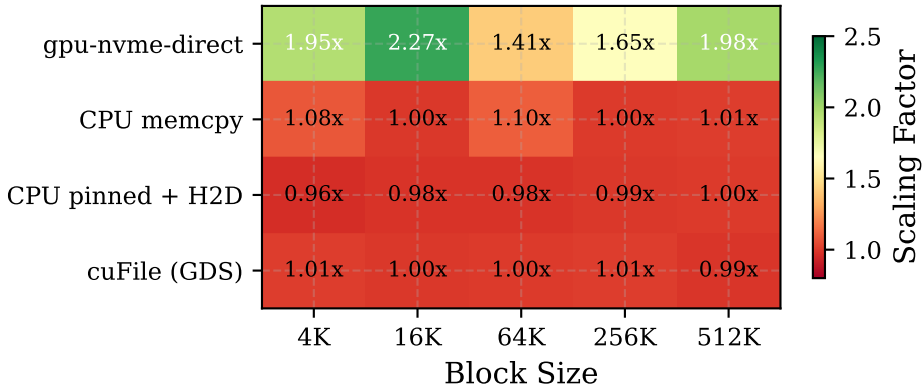
Throughput Scaling Factor (QD=32 / QD=1)
