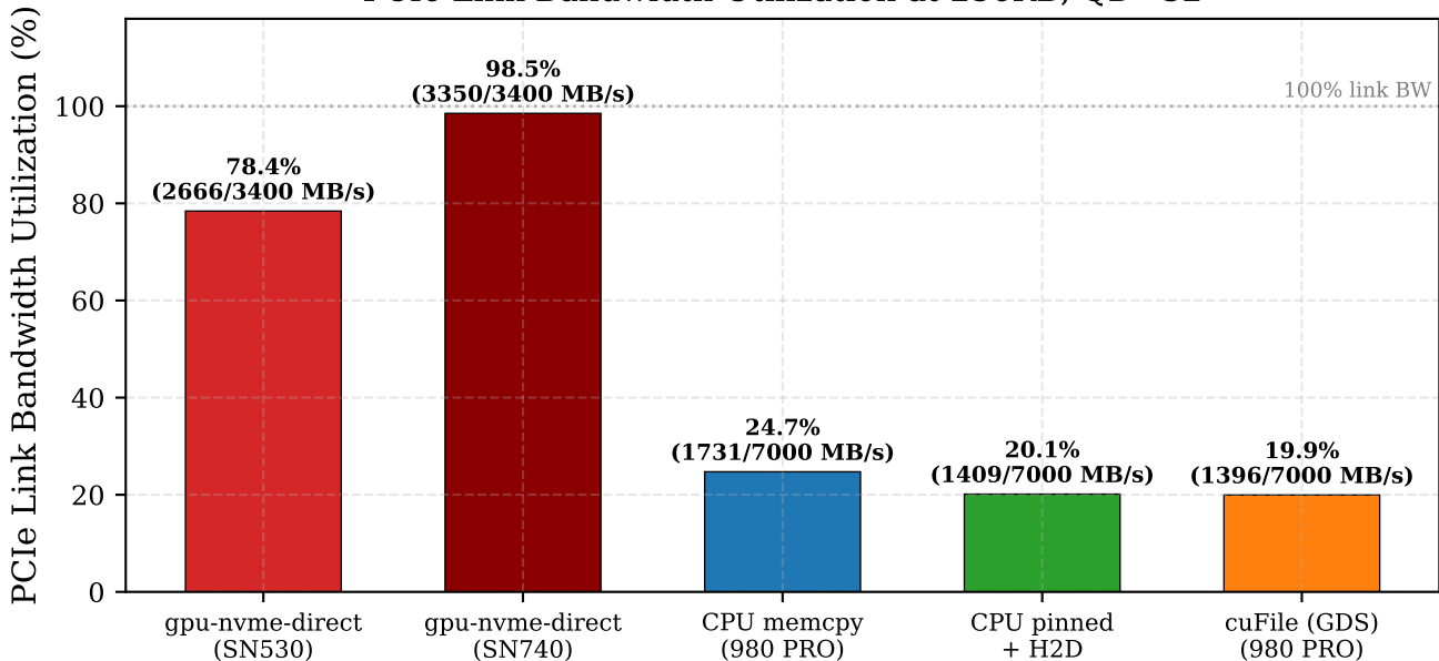
PCIe Link Bandwidth Utilization at 256KB, QD=32
