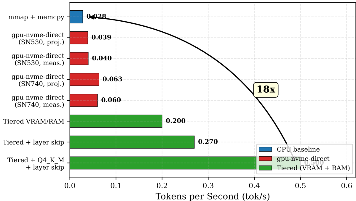
Llama-70B Inference: tok/s by Data Path
