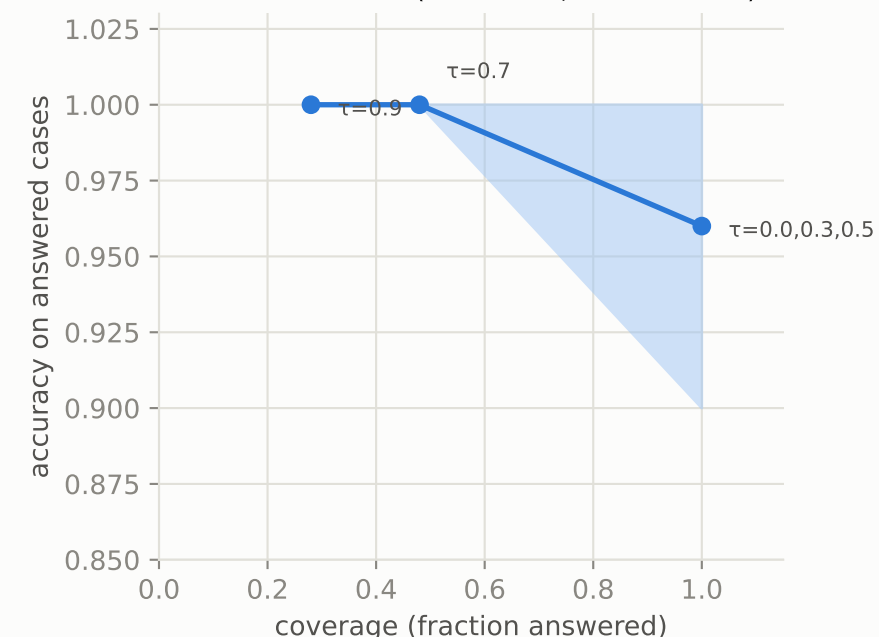
C. Deferral: accuracy vs coverage as abstain threshold \tau moves (monotone, 95% CI band)
