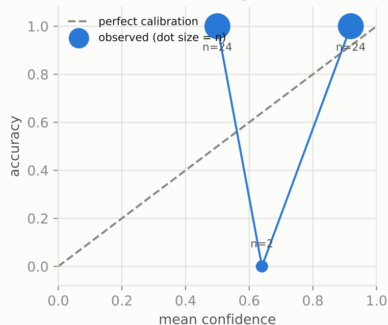
B. Calibration — ECE 0.304, Brier 0.141
