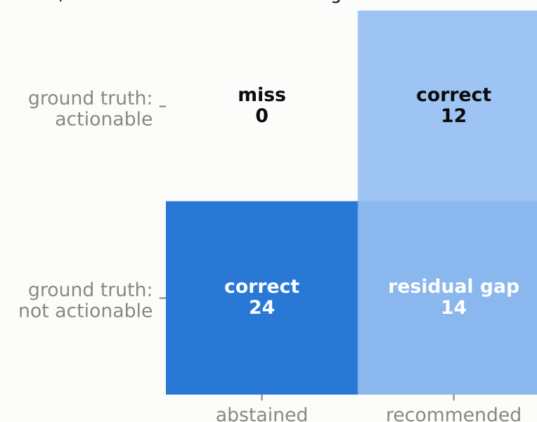
F. Abstention decision, post-fix (14/38 residual: guideline tier alone still clears the threshold — a gold-standard definition gap)
