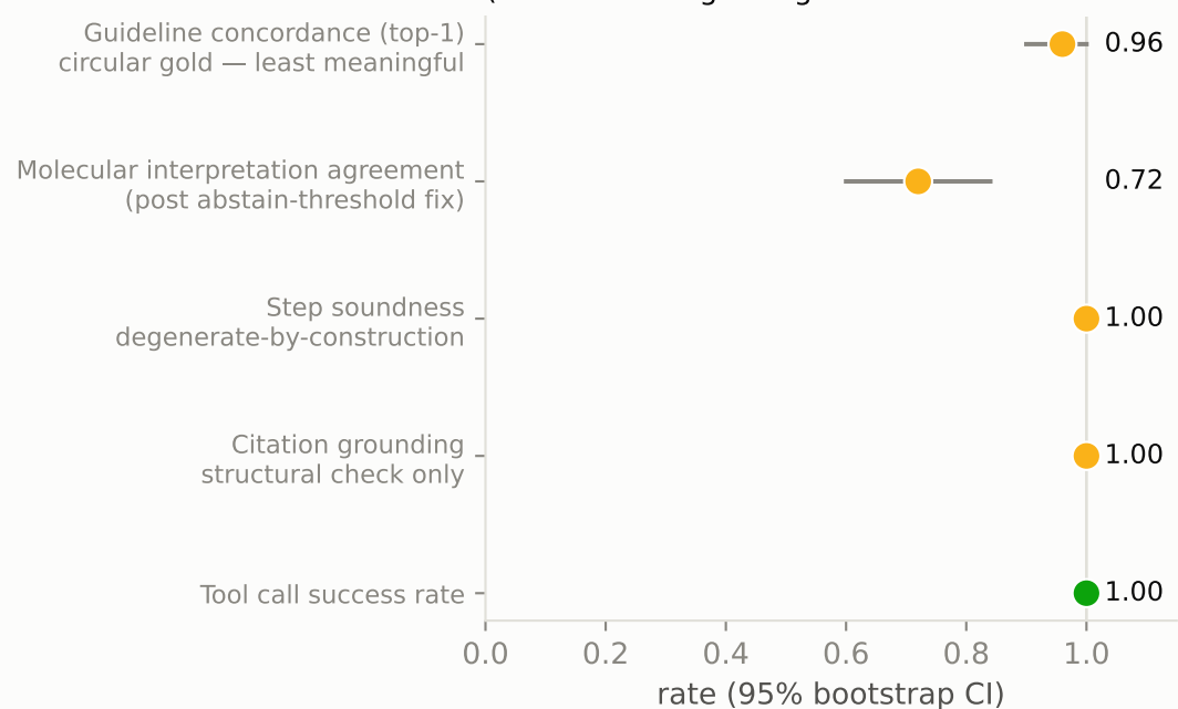
D. Headline metrics with bootstrap 95% CIs (color = read: green good · amber caveated · red concerning)
