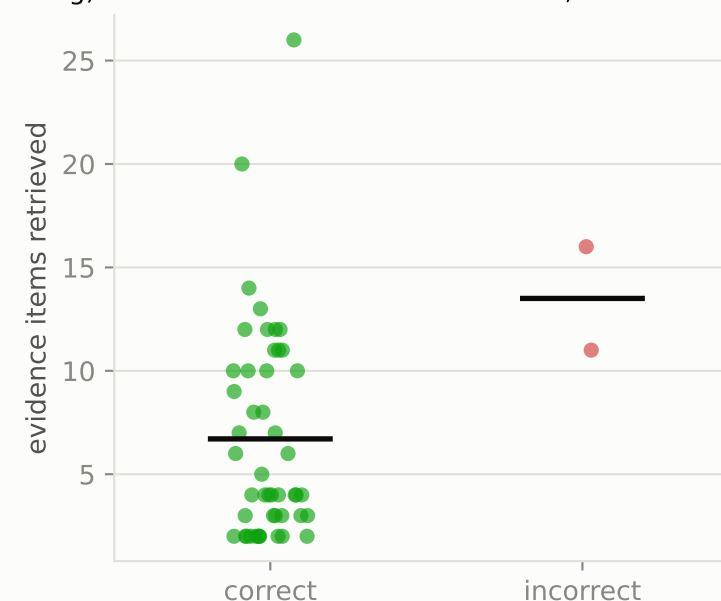
E. Information gathering — r = -0.256 ( p = 0.073 ) more evidence tracks with harder, not better-informed, cases
