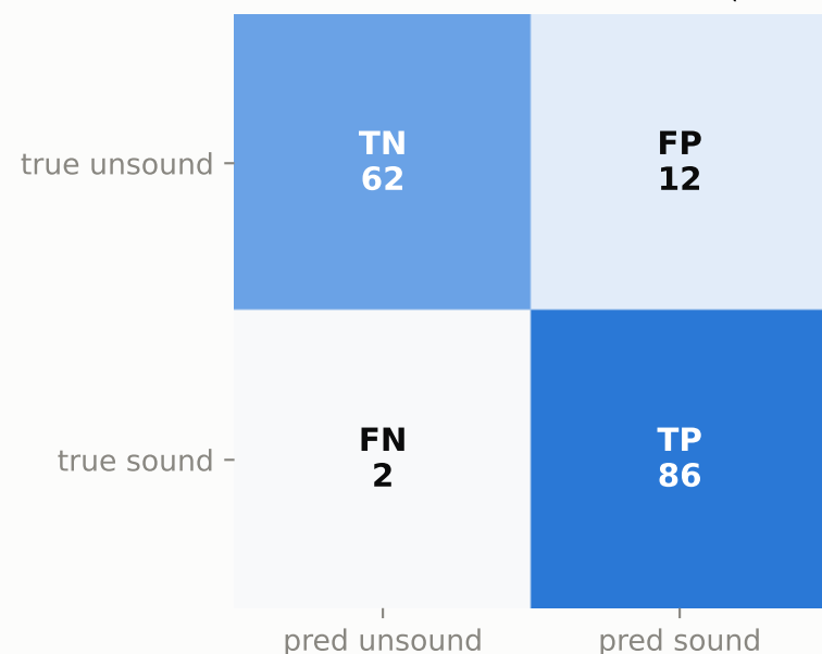
A. PRM held-out confusion matrix (acc 0.914)
