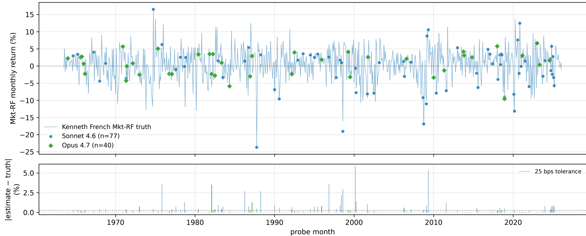
Sonnet 4.6 and Opus 4.7 recall the Mkt-RF series across 63 years
