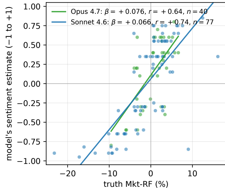
Sentiment vs ground truth
