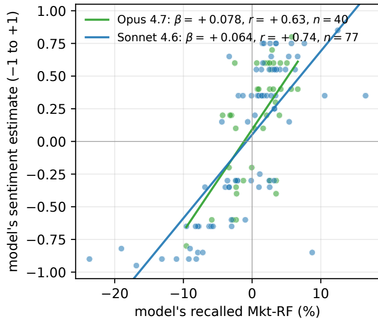
Sentiment vs model's own recall estimate
